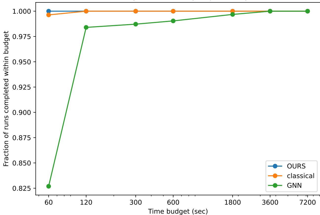
Coverage vs time budget (per family)
