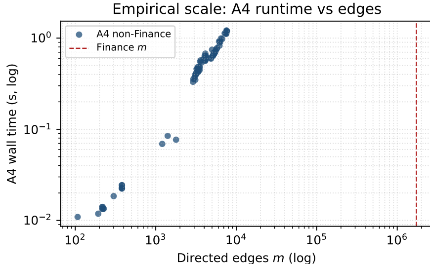
Figure 1: OURS-REACH (A4) wall time versus edge count on non-Finance graphs (log-log). Finance ( m \approx 1.73 \times 10^6 ) is marked as the large-dense boundary.
