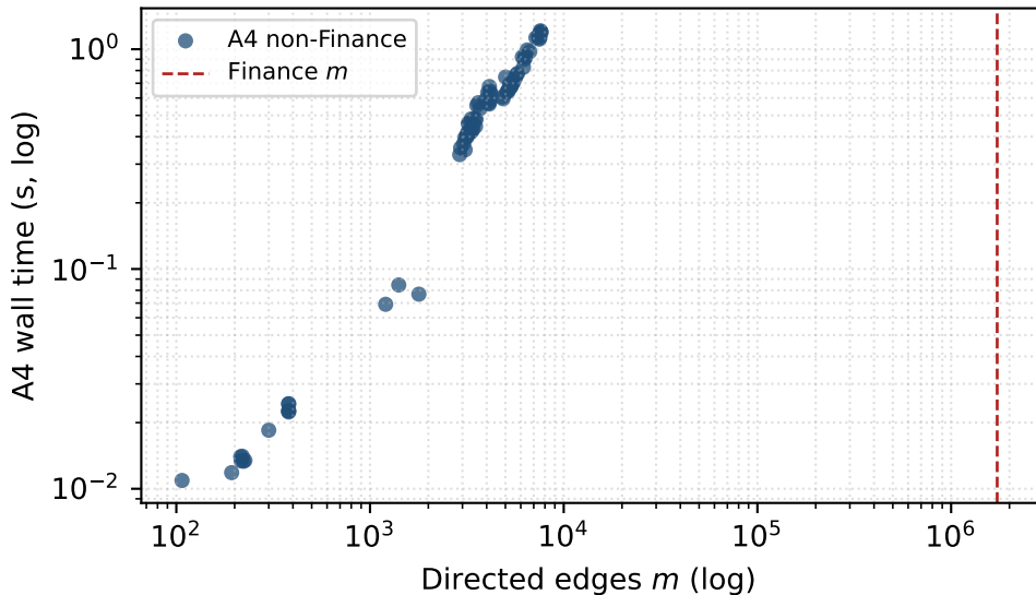
Empirical scale: A4 runtime vs edges
