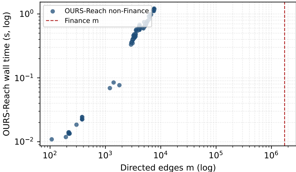
Empirical scale: OURS-Reach runtime vs edges
