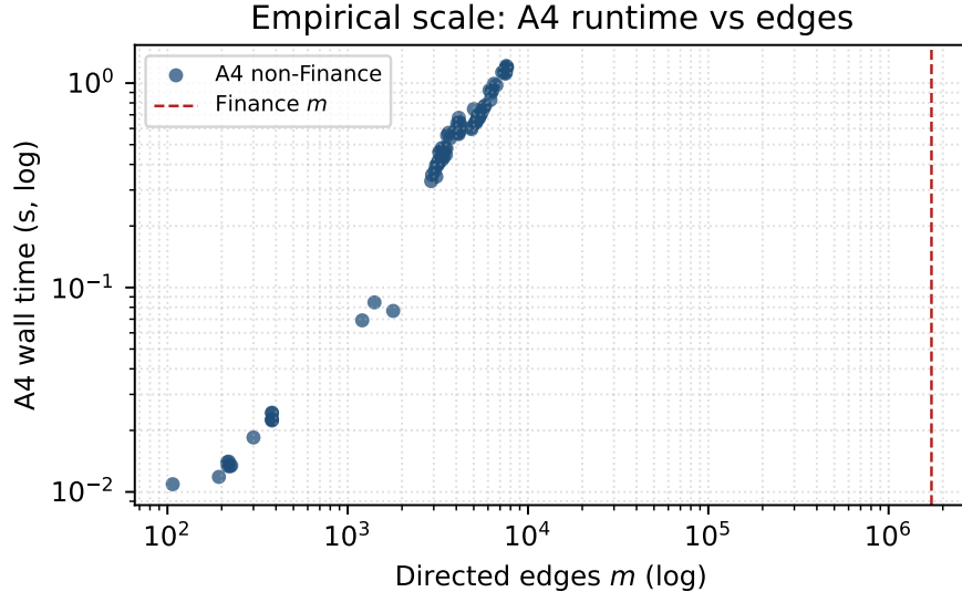
Figure 1: OURS-REACH wall time versus edge count on non-Finance graphs (log-log). Finance ( m \approx 1.73 \times 10^6 ) is marked as the large-dense boundary.
