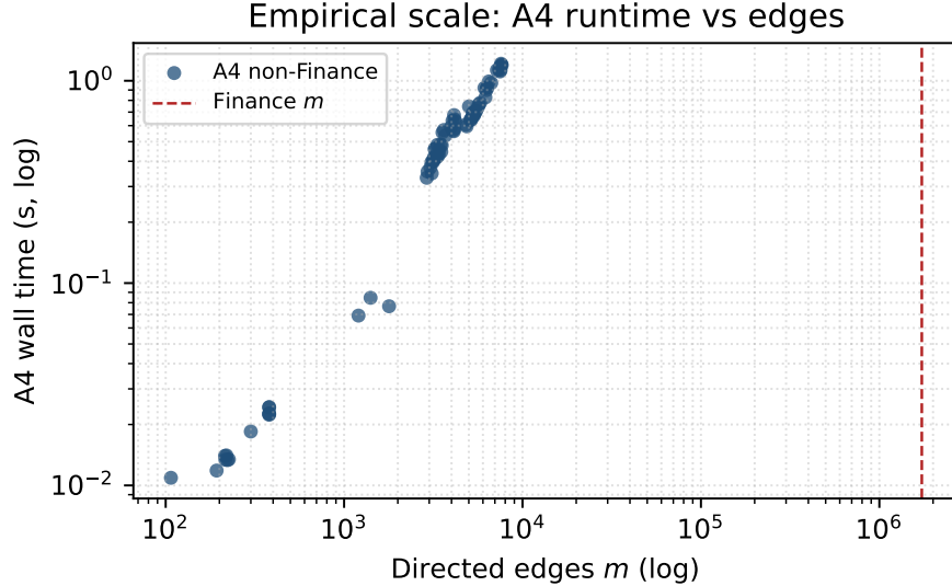
Figure 1: A4 wall time versus edge count on non-Finance ablation graphs (log-log). Finance ( m \approx 1.73 \times 10^6 ) is marked as the large-dense boundary.
