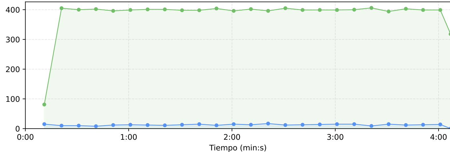
Requests State
