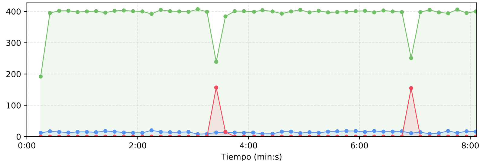
Requests State
