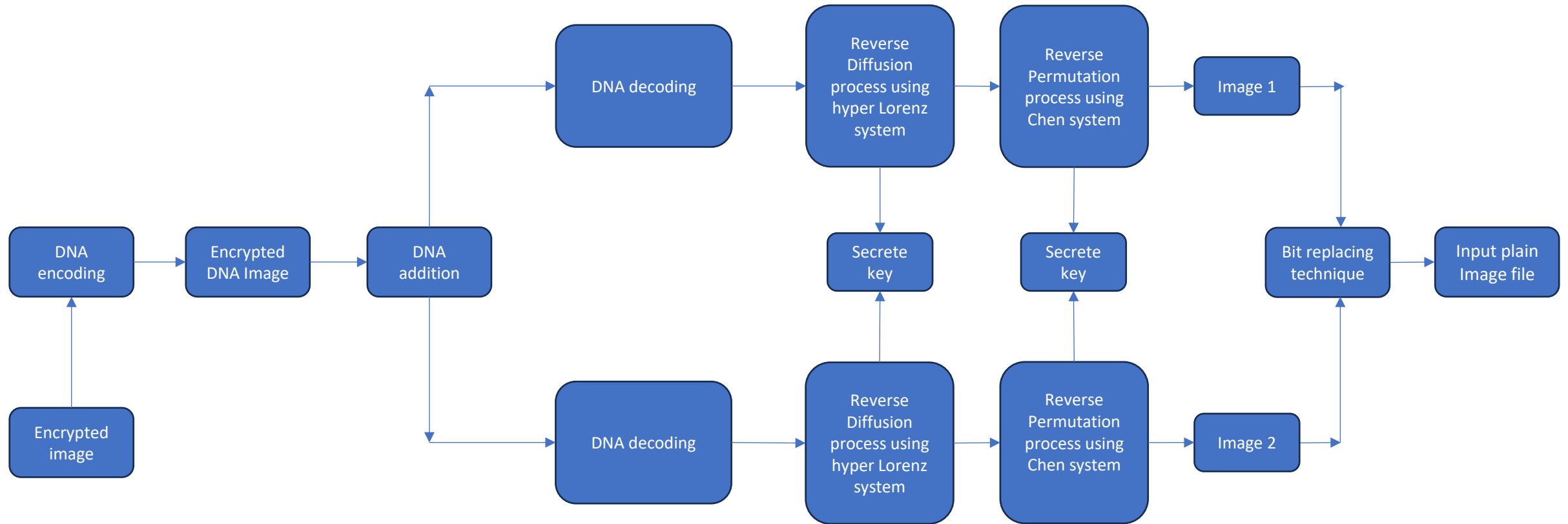
Fig. decryption algorithm block diagram/flowchart
