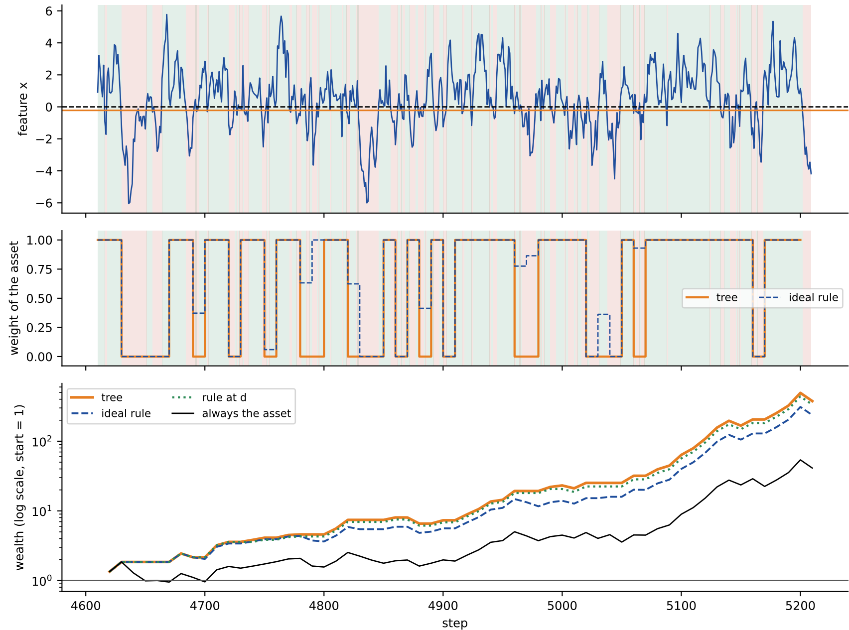
Test period, never seen in training: the regimes (green/red), the tree's threshold (orange) and its decisions
