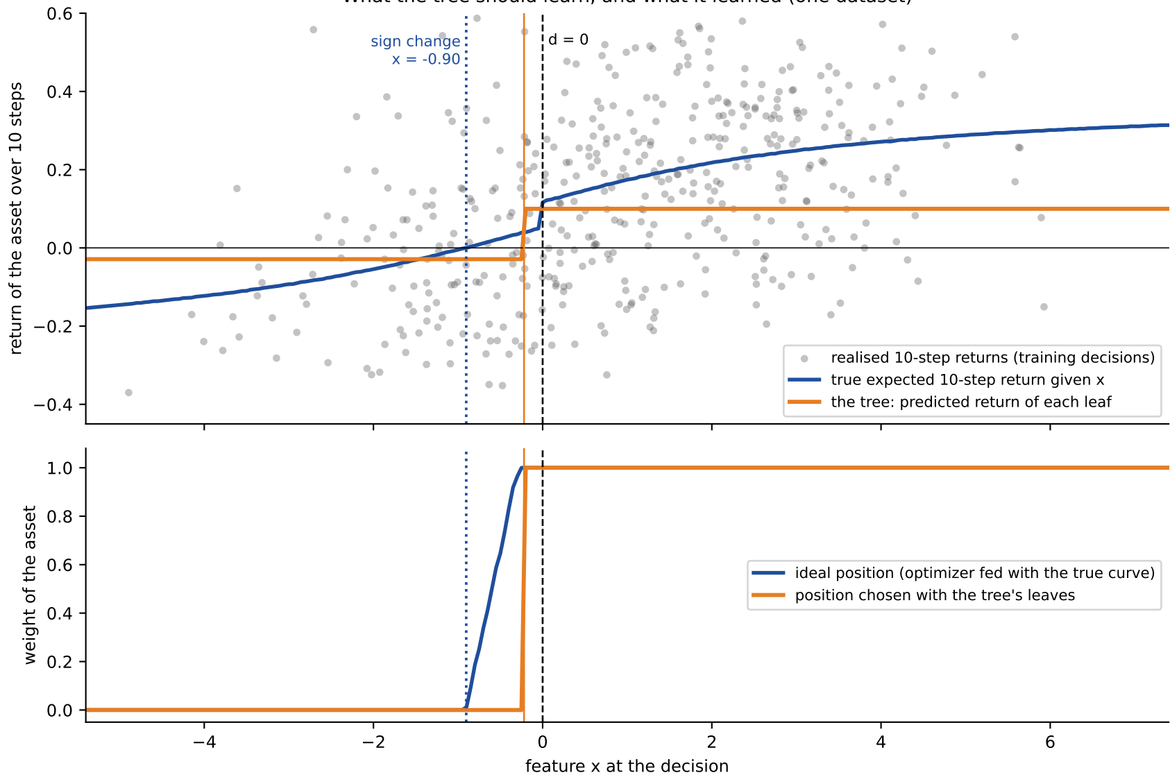
What the tree should learn, and what it learned (one dataset)
