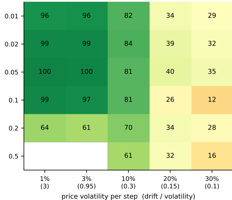
test gain over the tree without splits, as % of the ideal rule's gain (blank: nothing to gain)
