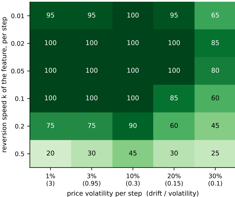
first split on the true feature x (% of 20 datasets)
