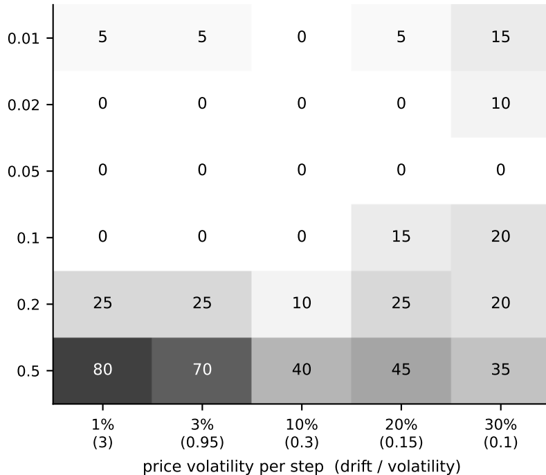
no split kept after pruning (% of 20 datasets)
