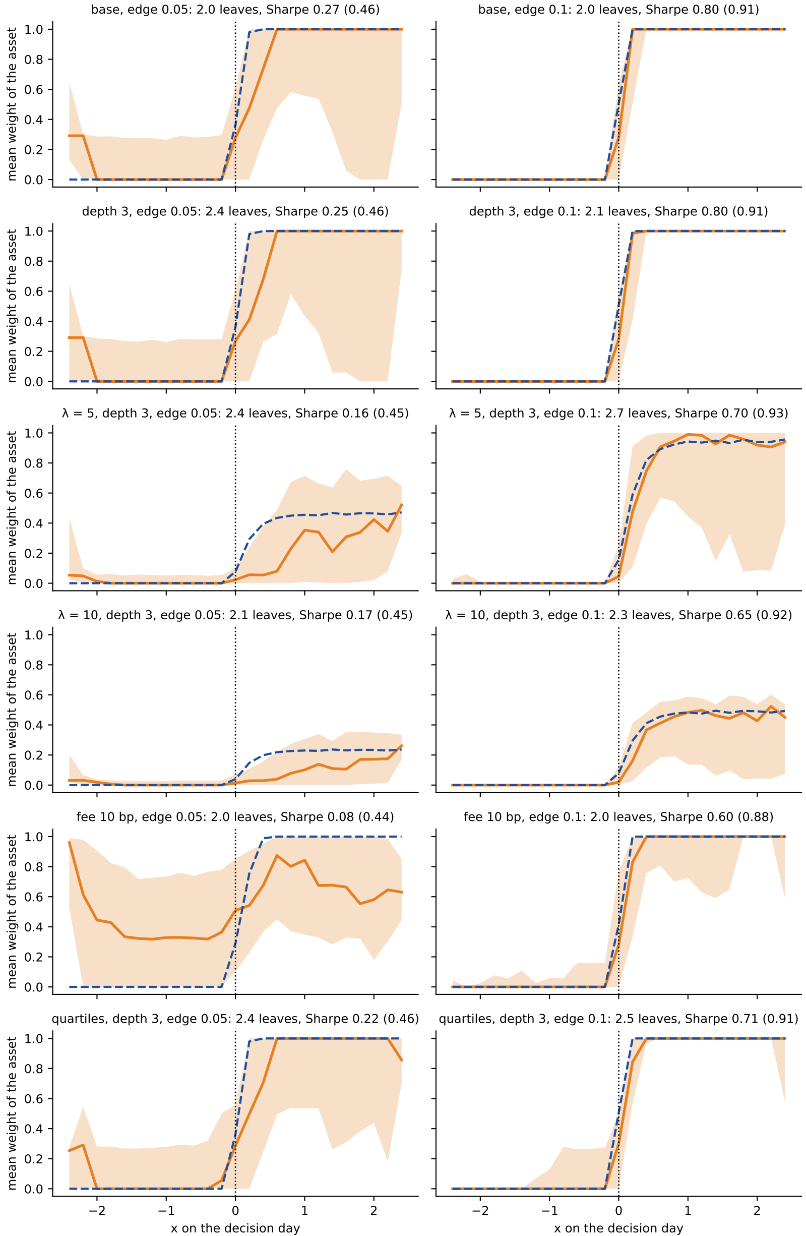
Position taken on the test decisions, by x (weekly decisions, 40 datasets per panel)
