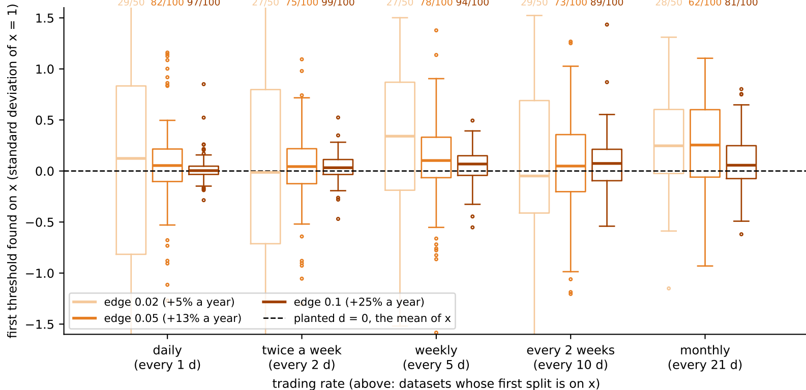
Threshold found against the trading rate and the strength of the drift ( k = 0.02 , volatility 1% a day)
