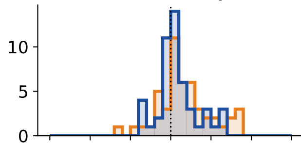
half-life 6.9 days
