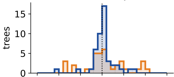
half-life 2 days
