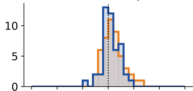
half-life 69 days
