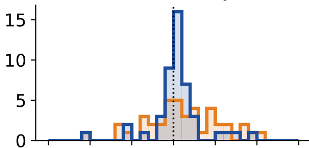
half-life 3.5 days
