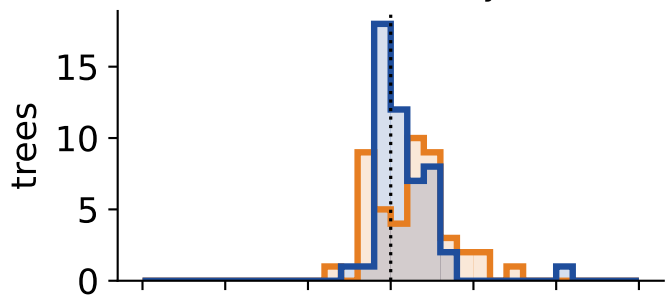
half-life 14 days
