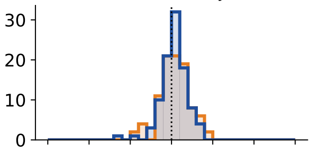
half-life 35 days
