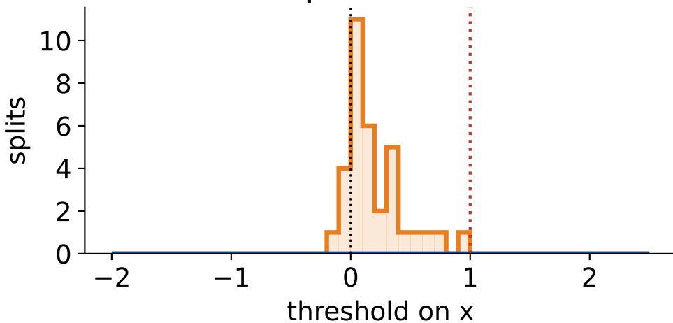
\lambda = 10 , 20-day covariance, 40 datasets 0% split near d + 1
