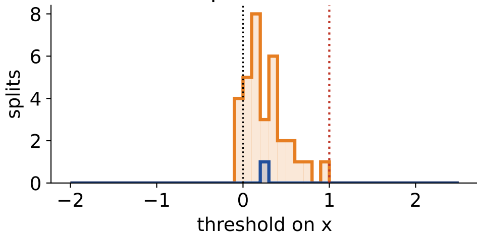
\lambda = 10 , 180-day covariance, 40 datasets 0% split near d + 1
