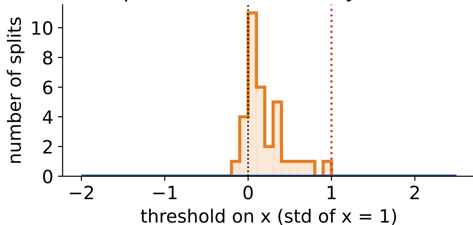
\lambda = 10 , 20-day covariance (40 datasets) 0% split near the volatility threshold
