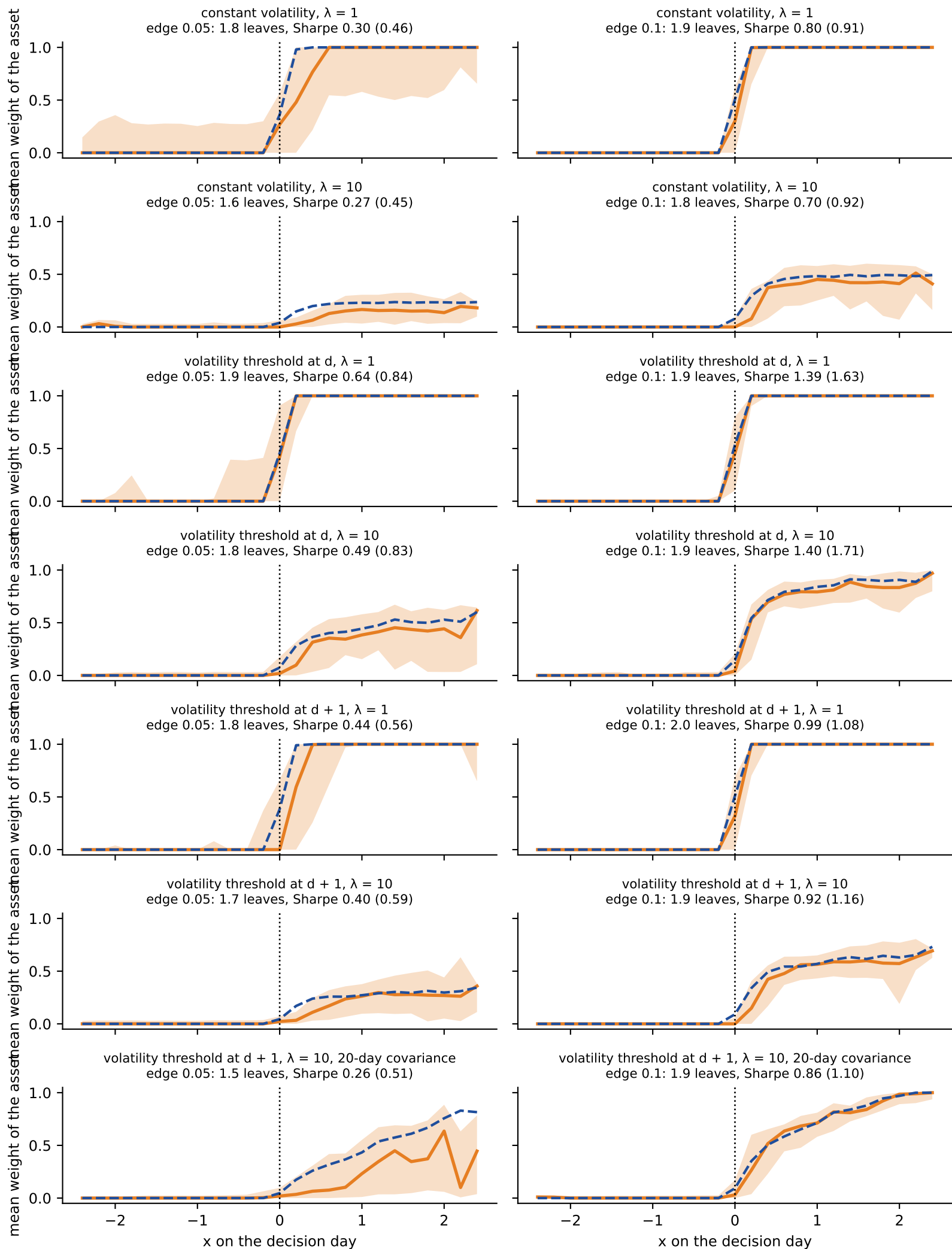
Position taken on the test decisions, by x (weekly decisions, 40 datasets per panel)
