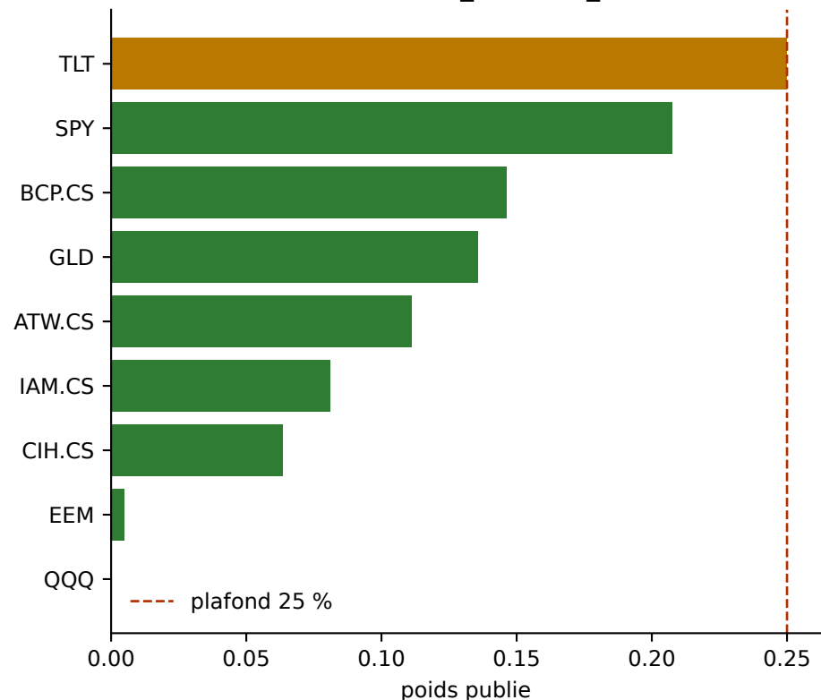
Systeme primaire : trace deterministe bear -> min_variance_lw
