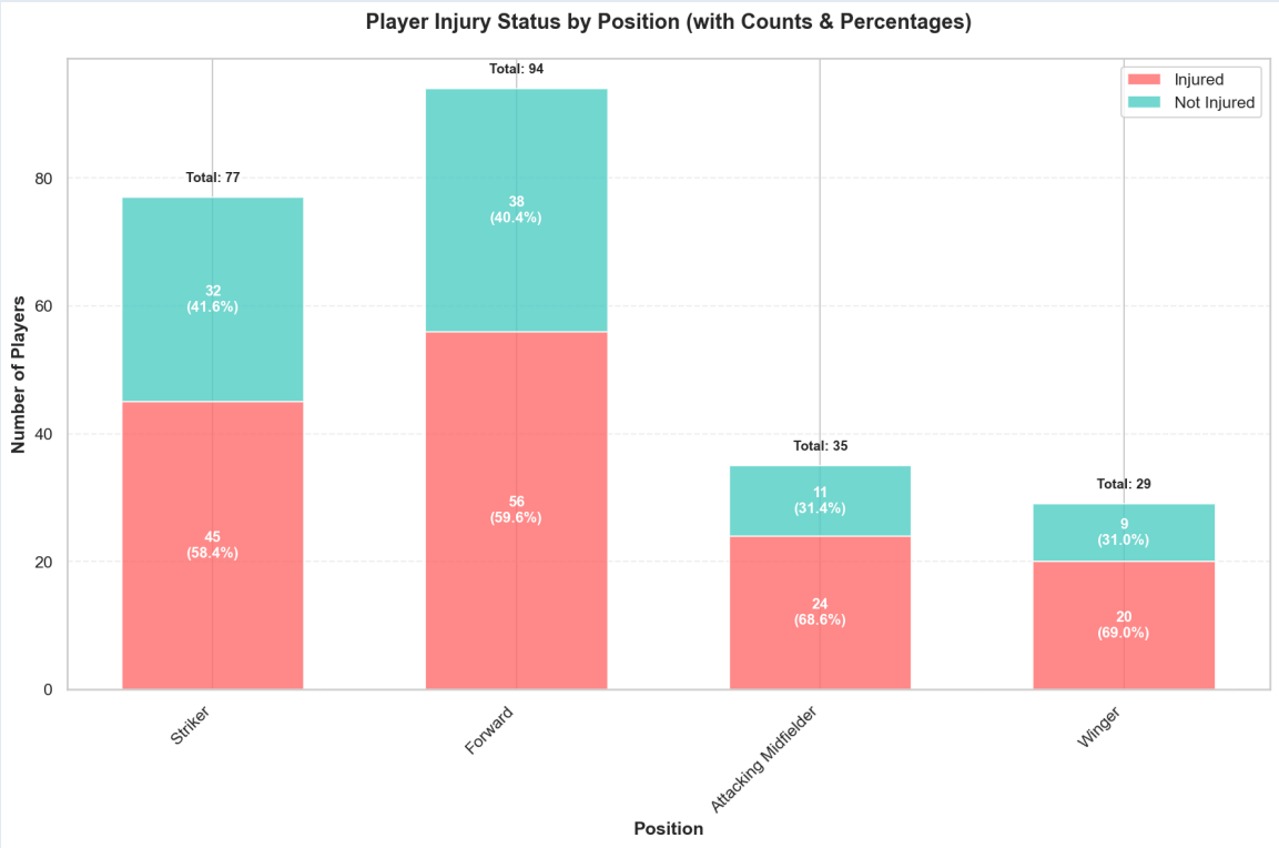
Figure: Football Injuries by Position.
