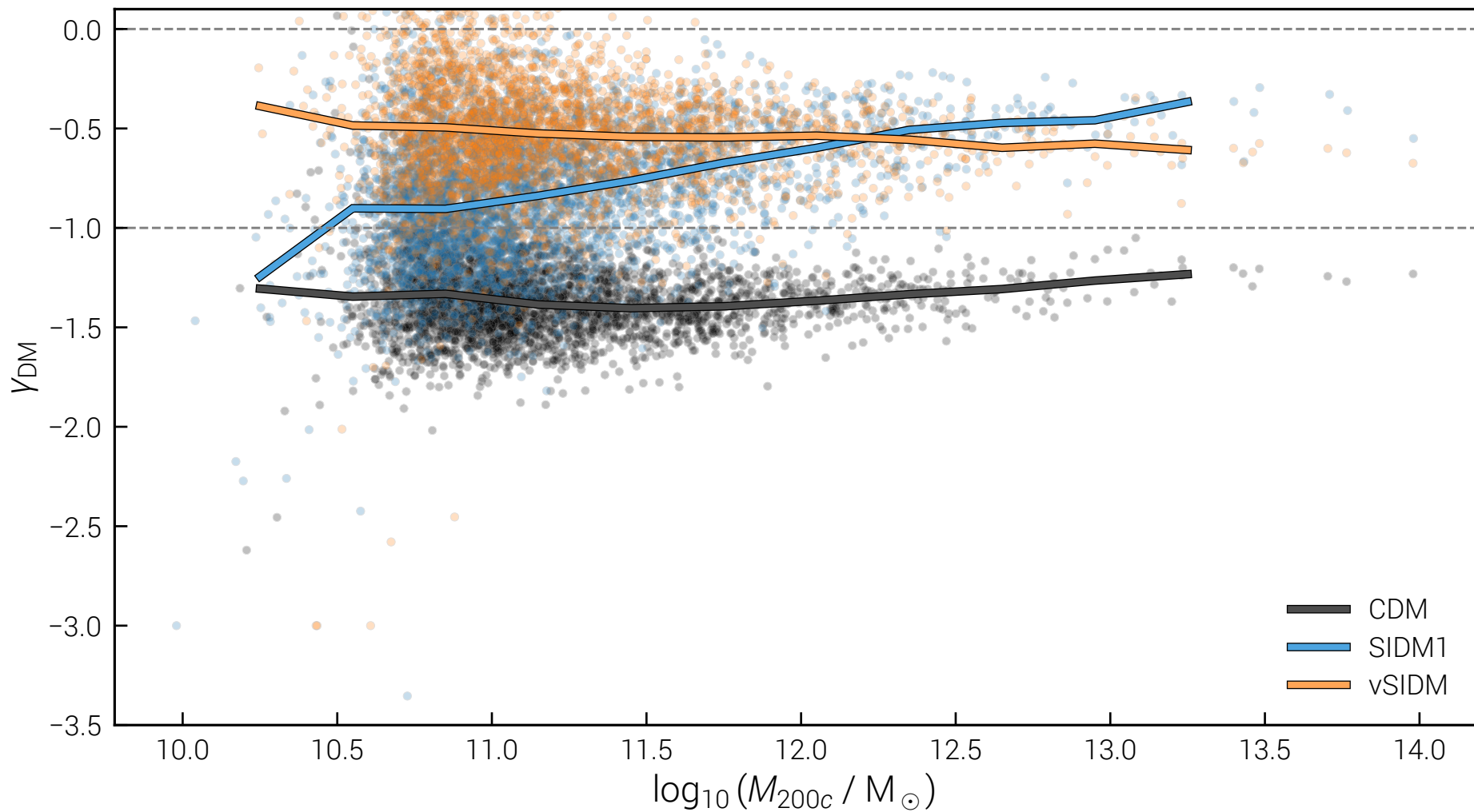
Inner DM density slope (DMO, z=0.5 )
