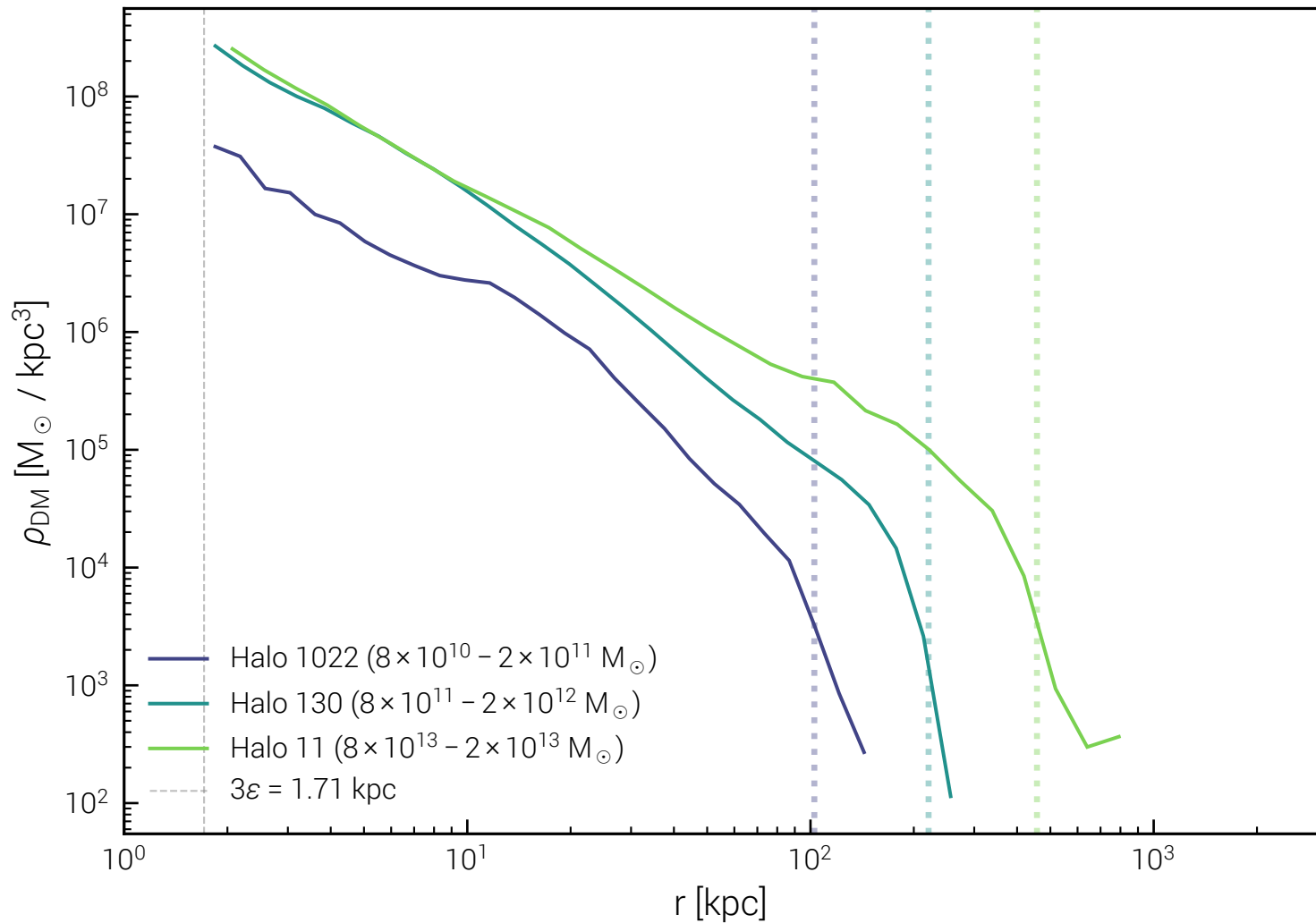
CDM DM density profiles (z=0.5)
