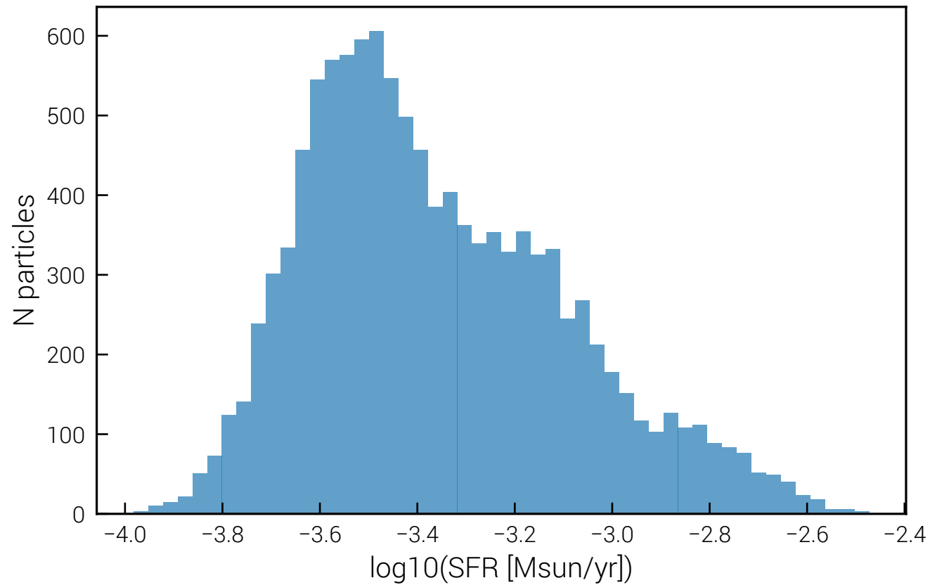
SFR distribution (FoF 200, snap 67)
