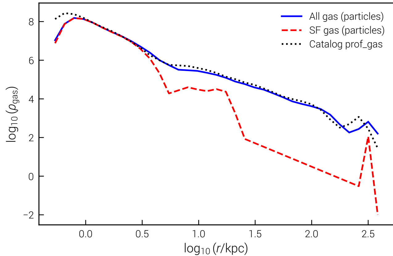
Gas density profiles
