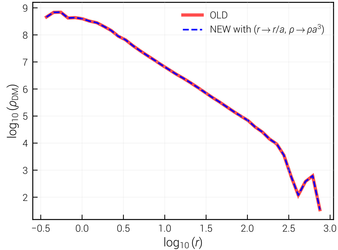
After undoing a-scaling: exact overlay
