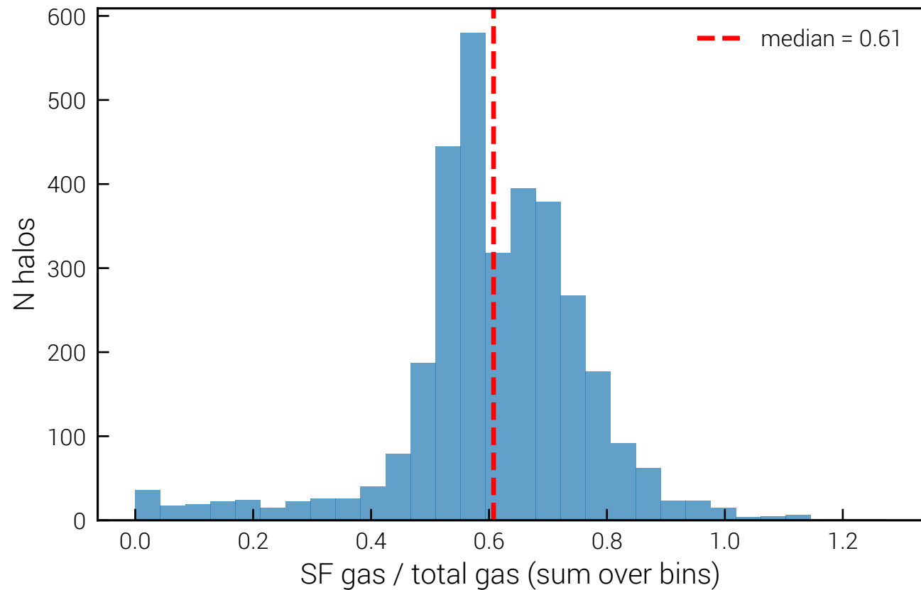
CDM snap 67 (z=0.50): SF gas fraction
