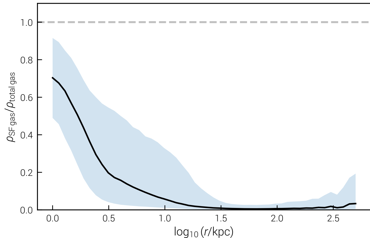
SF gas fraction vs radius (median + 16-84 pct)
