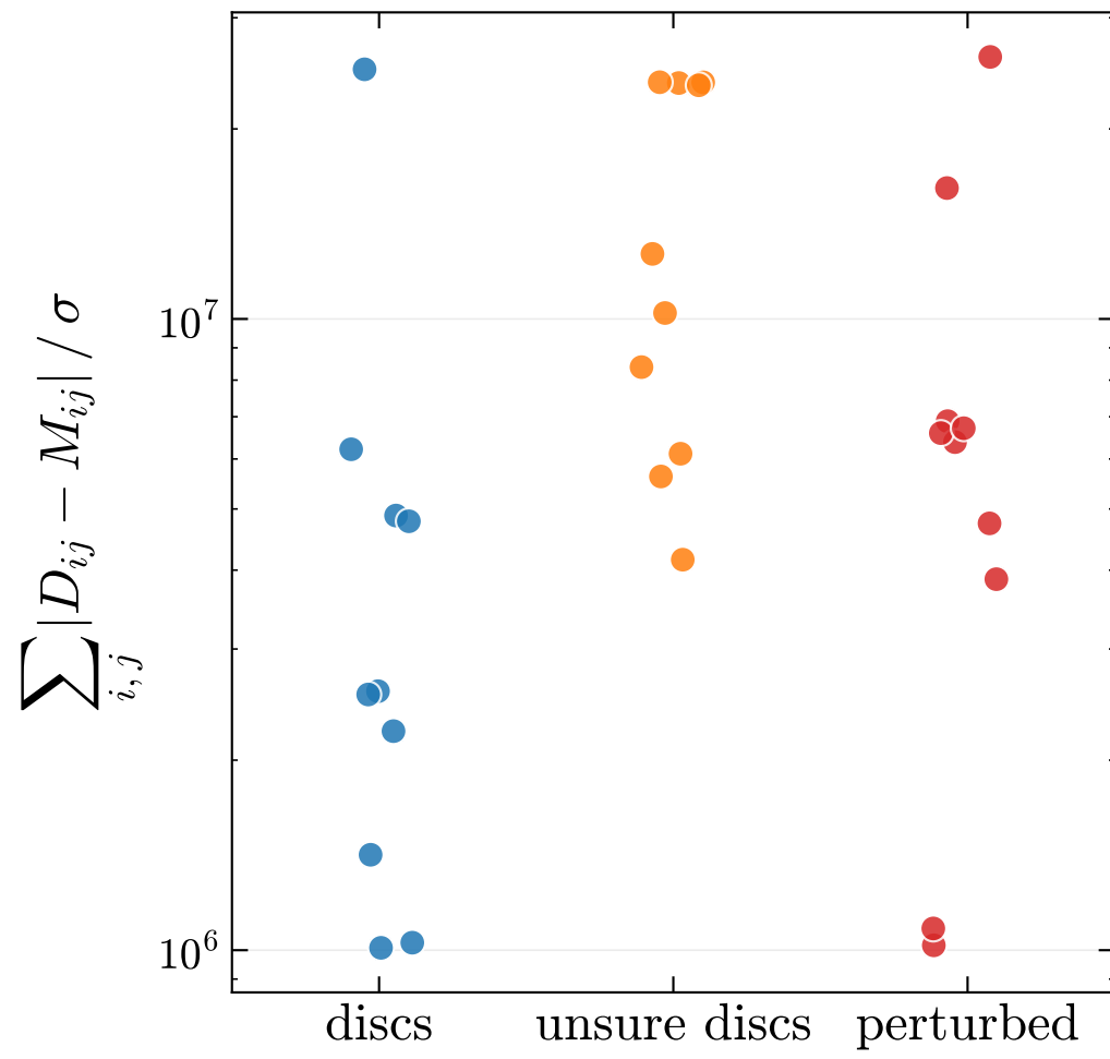
Cube (CDM, z = 0.5 )
