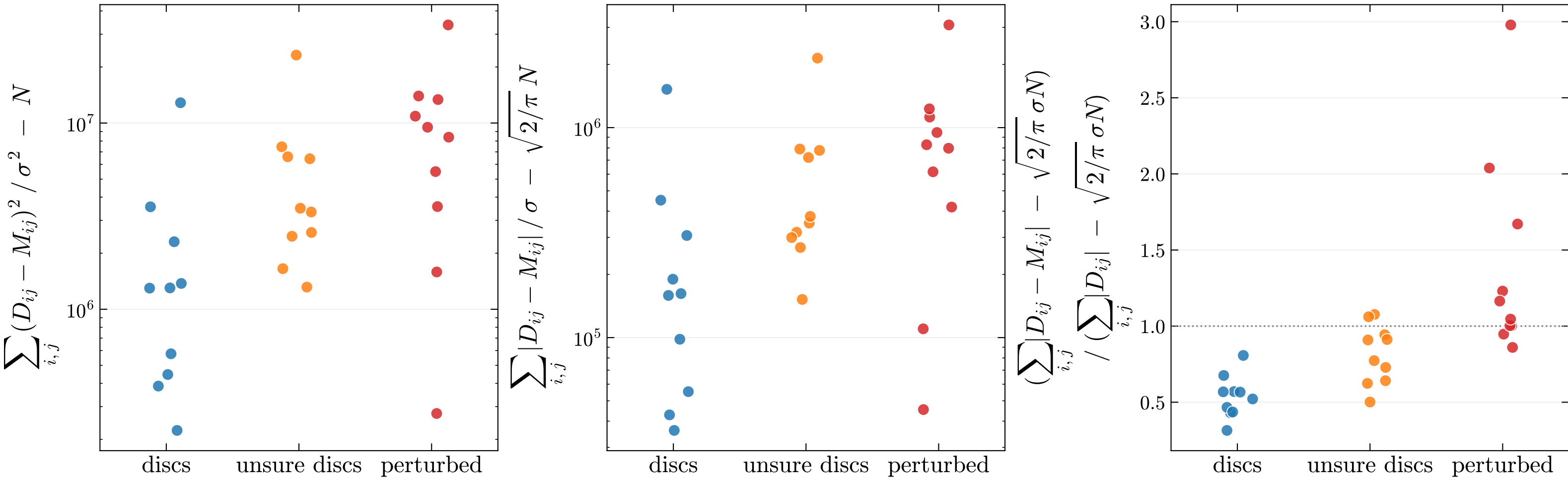
Cube, noise floor subtracted (CDM, z = 0.5 )
