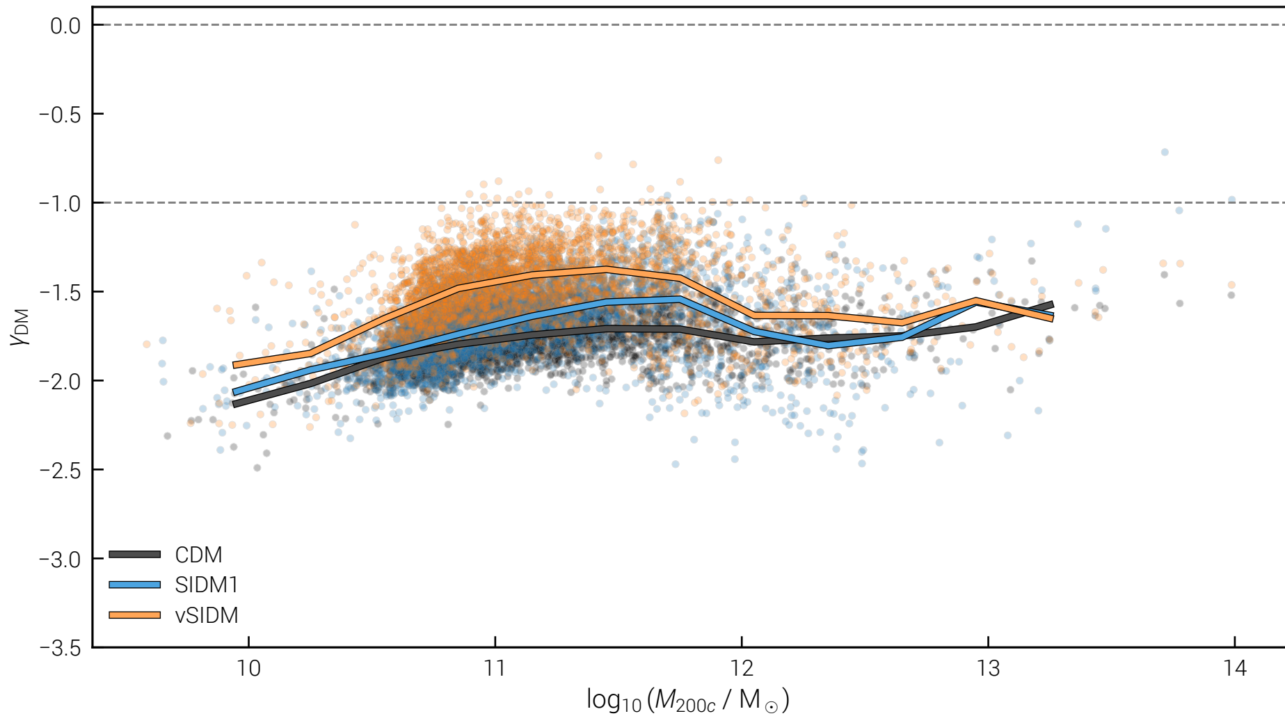
Inner DM density slope (FP, z=0.5 )
