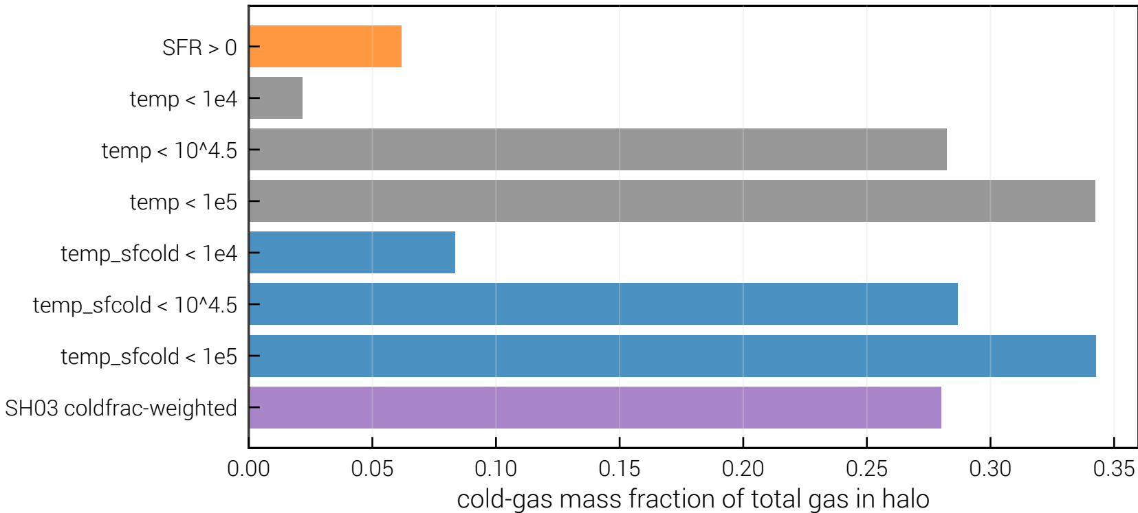
CDM halo 85: cold-gas mass fraction vs definition
