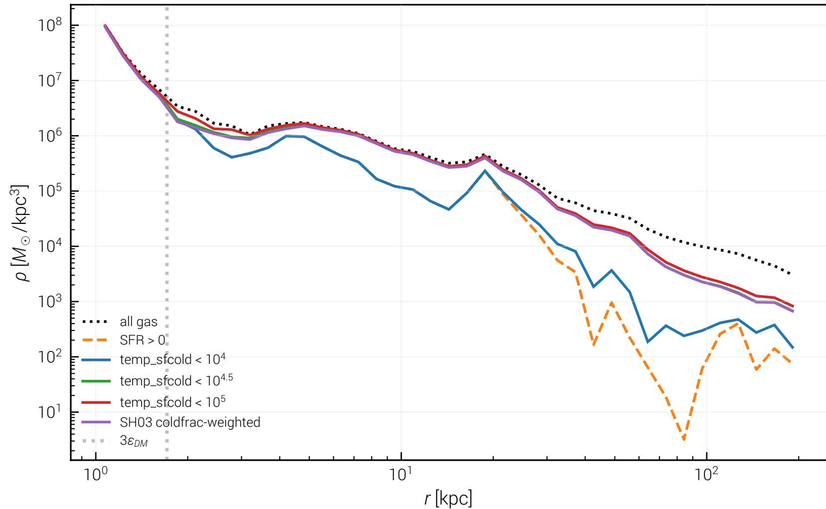
CDM halo 85 - gas density under different cold-gas definitions
