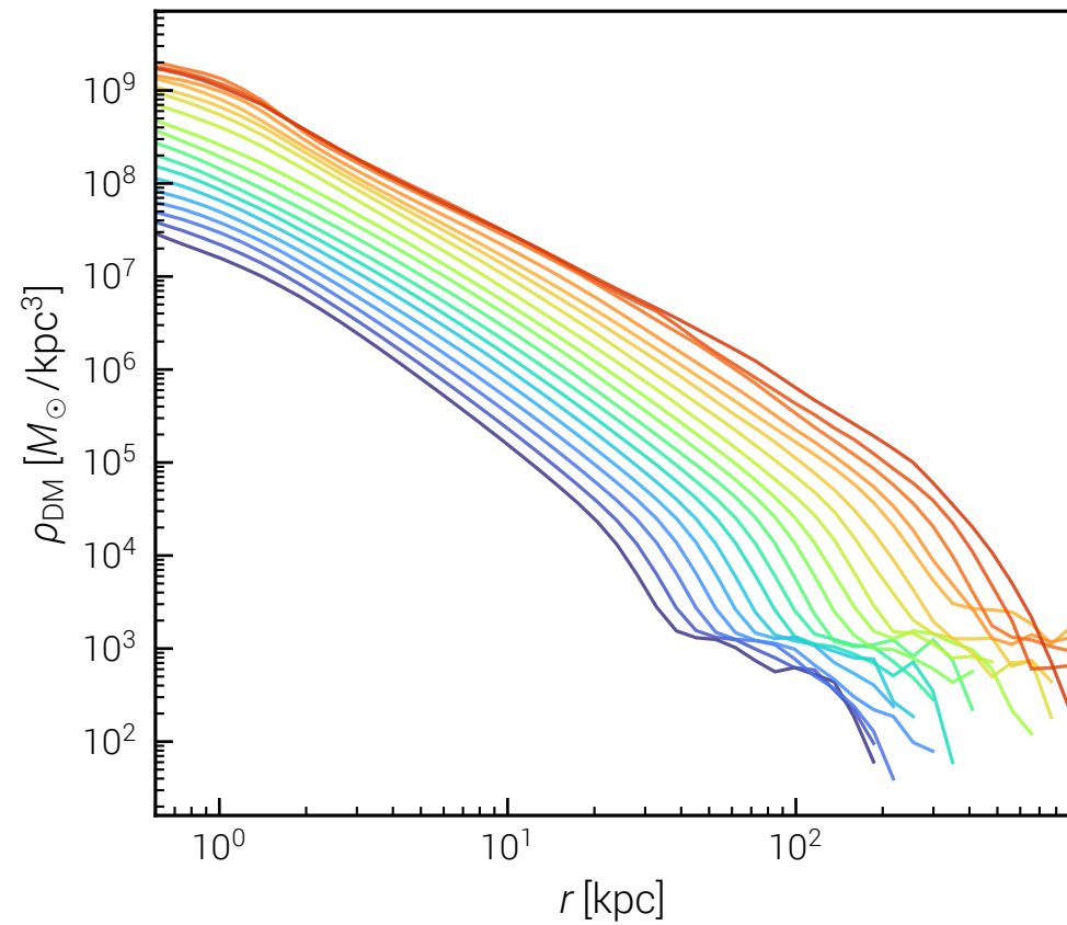
CDM
