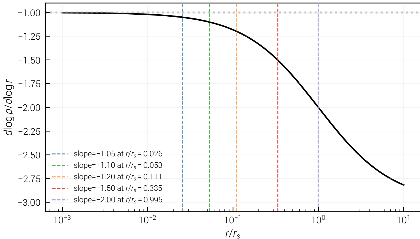
NFW log-slope vs radius
