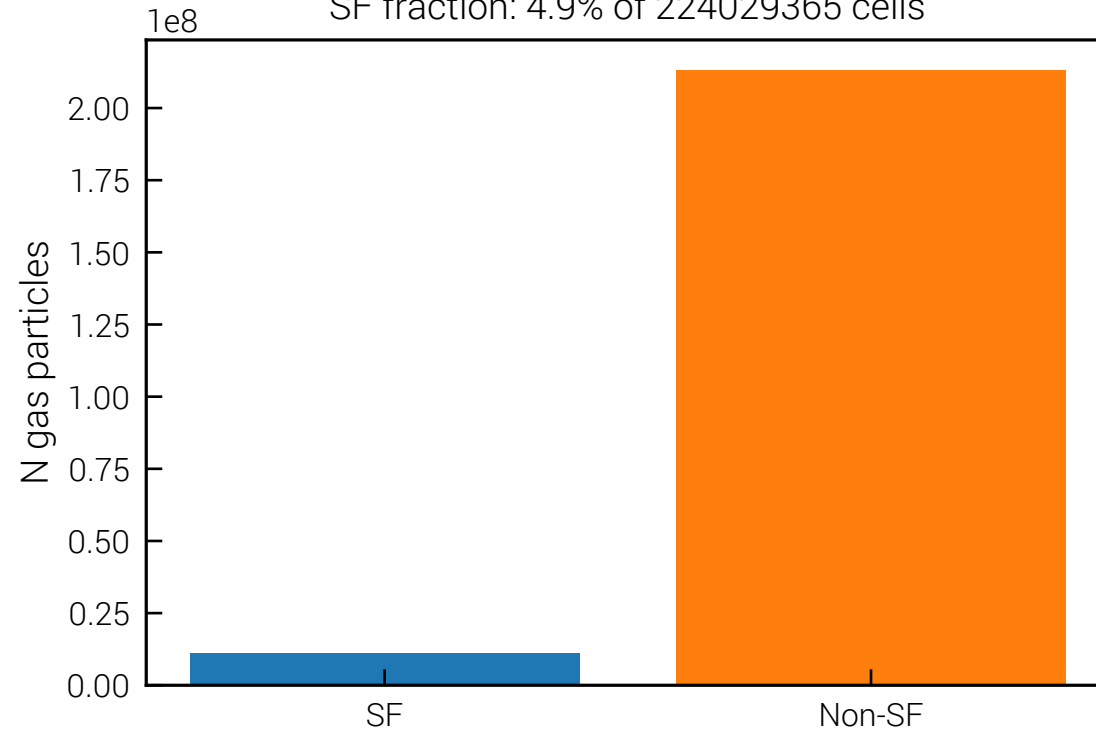
SF fraction: 4.9% of 224029365 cells
