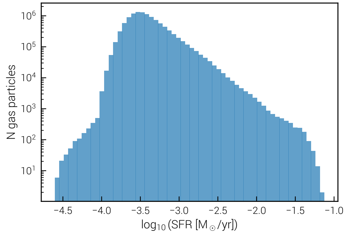
SFR per cell (SF cells only)
