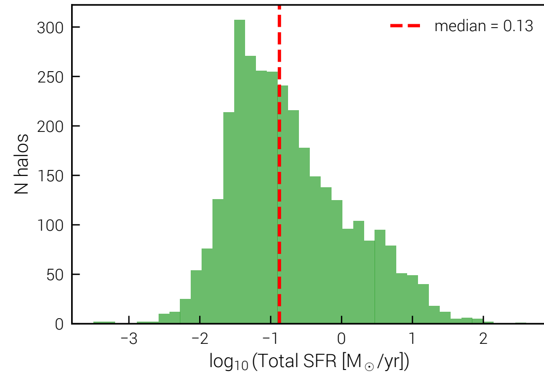
Total SFR per halo (3308/3355 with \text{SFR} > 0 )
