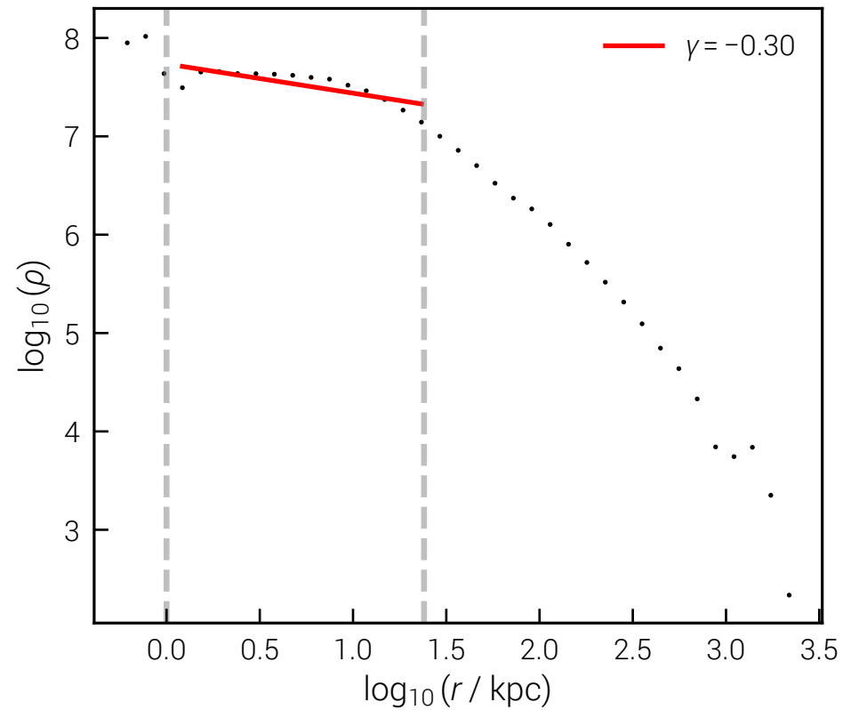
\sim 10^{14} vSIDM DMO FoF 0, \log M = 14.0
