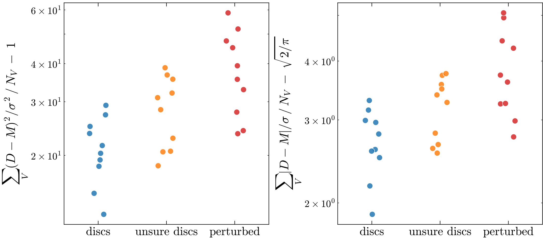
Cube (CDM, z = 0.5 )
