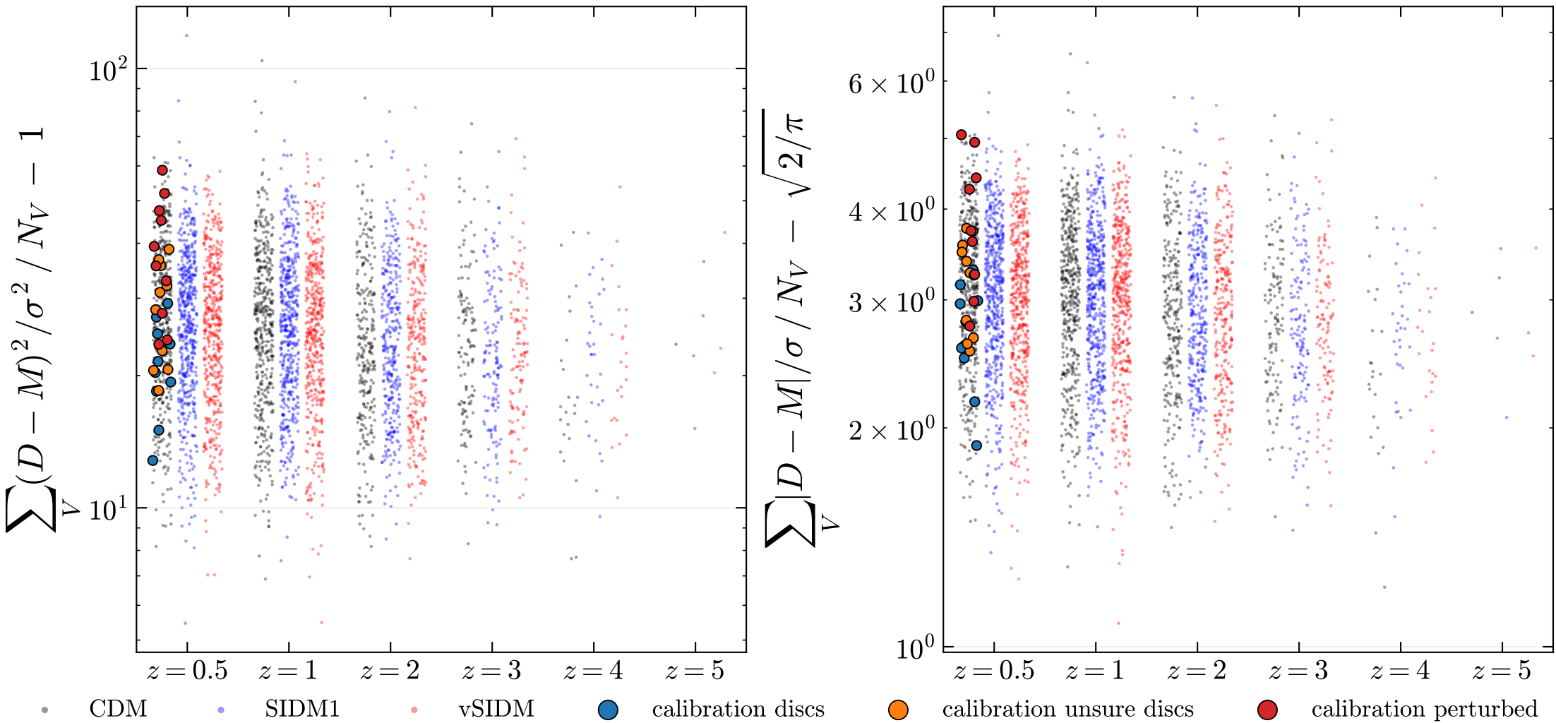
Cube, all galaxies
