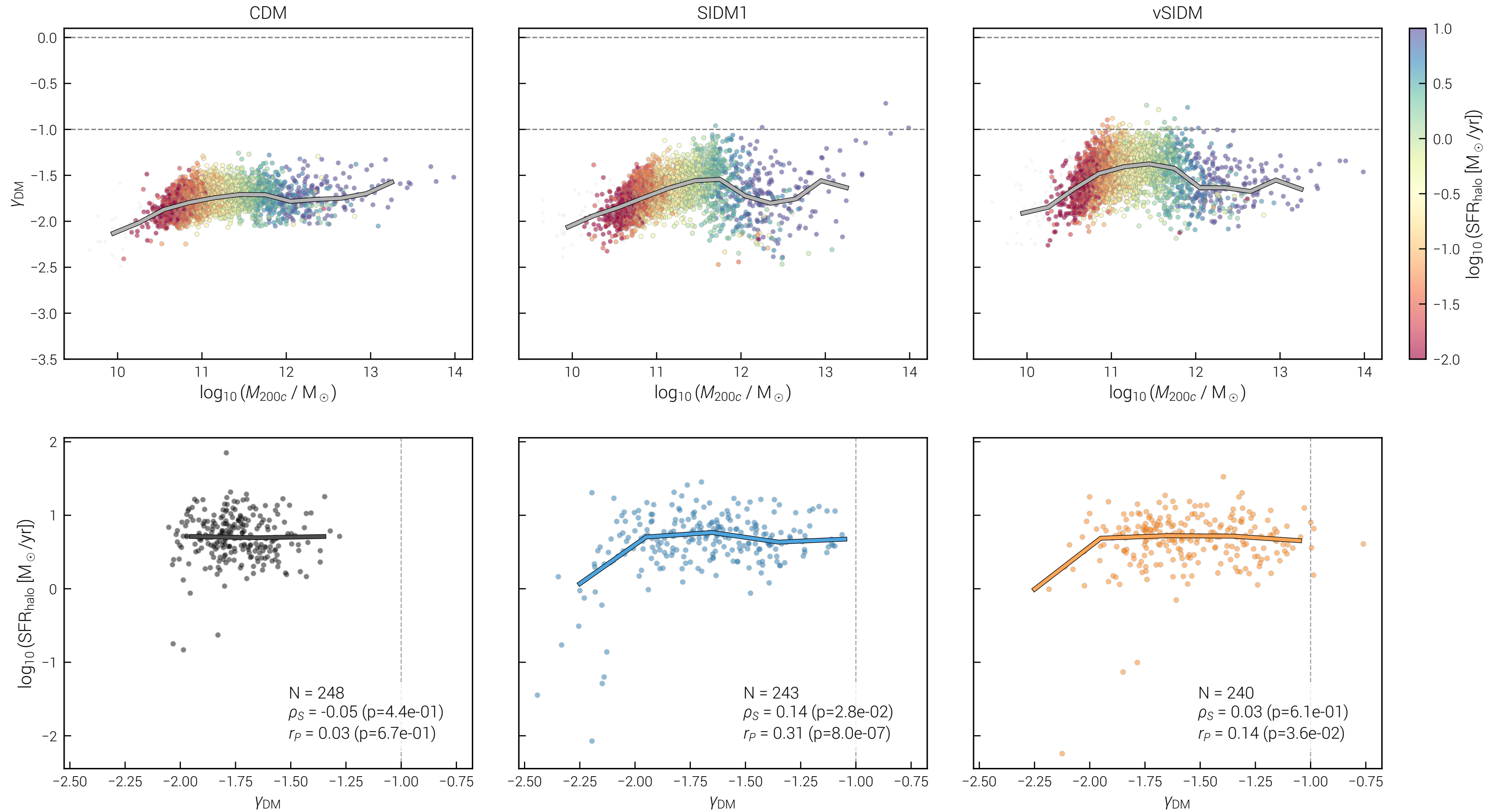
halo-scope SFR; \log_{10}(M_{200c}) = 12.0 \pm 0.25 (bottom row), z=0.50
