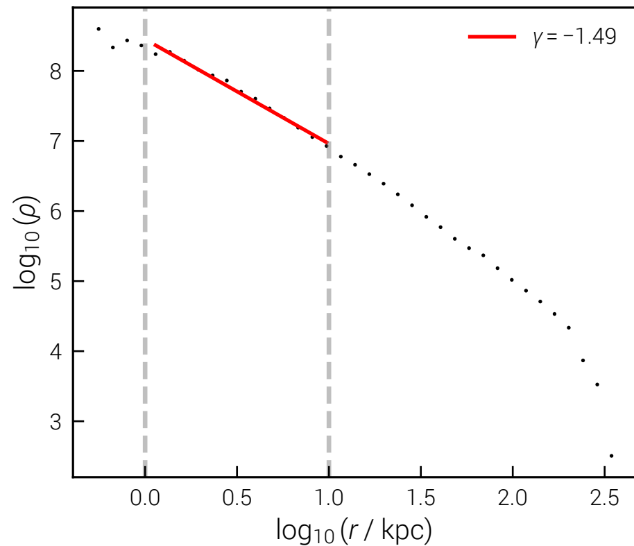
\sim 10^{12} CDM DMO FoF 117, \log M = 12.3
