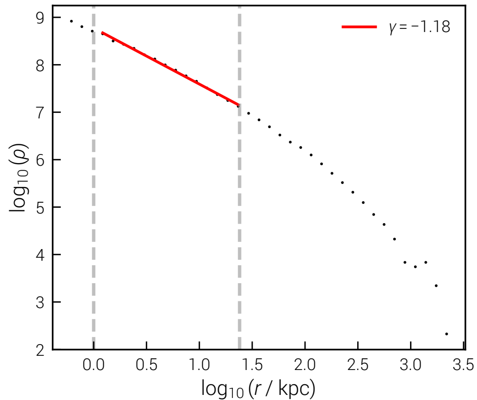
\sim 10^{14} CDM DMO FoF 0, \log M = 14.0
