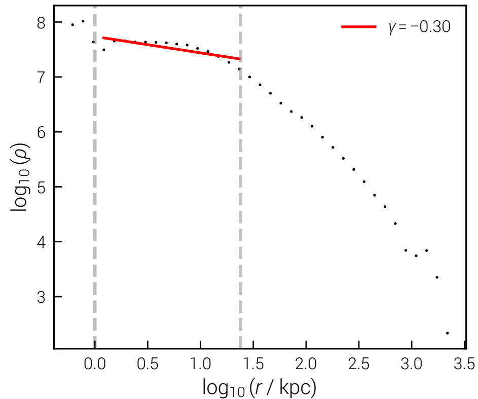
\sim 10^{14} vSIDM DMO FoF 0, \log M = 14.0
