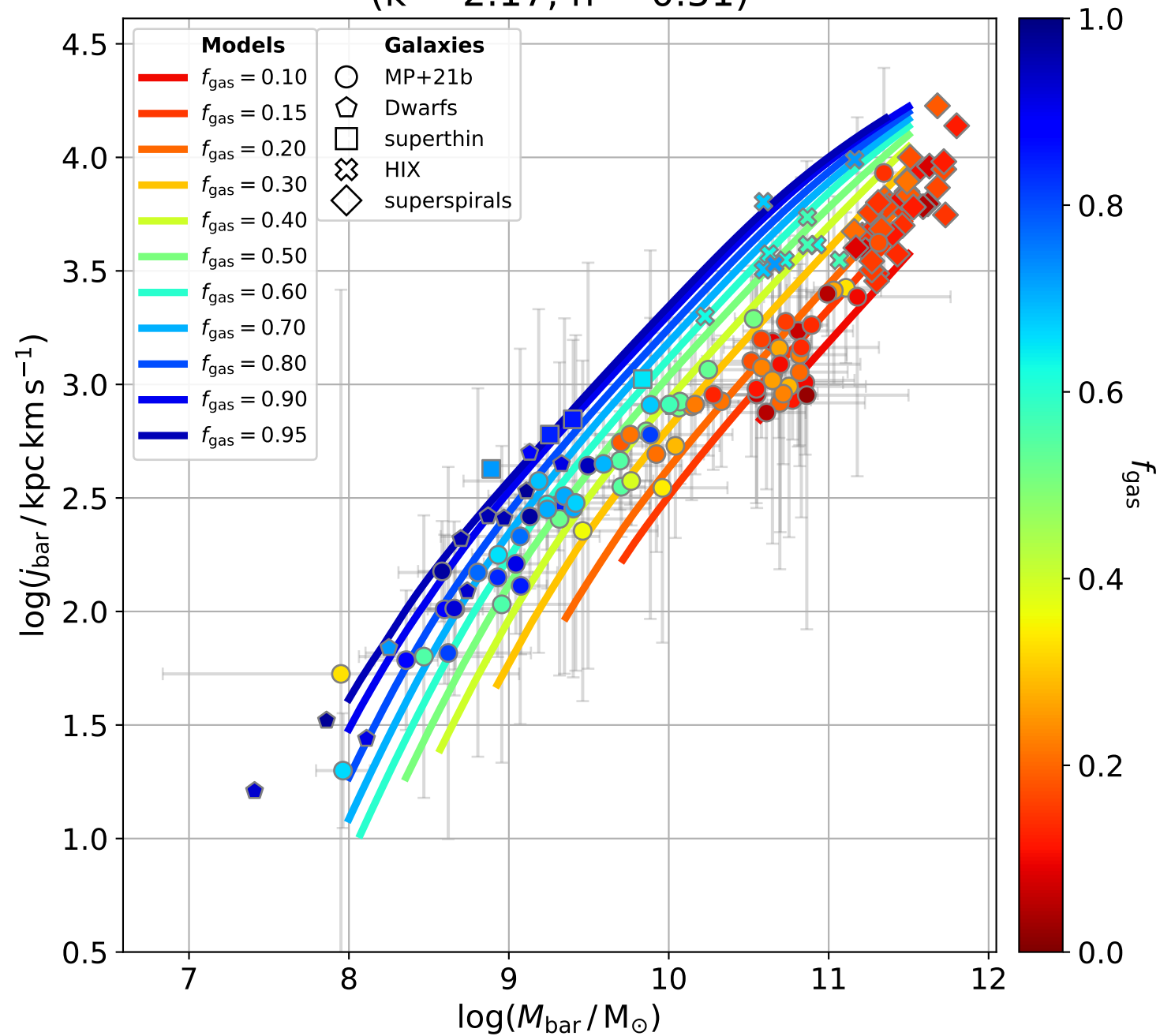
\log(j_{\text{bar}}) vs \log(M_{\text{bar}}) vs f_{\text{gas}} ( k = 2.17 , n = 0.51 )
