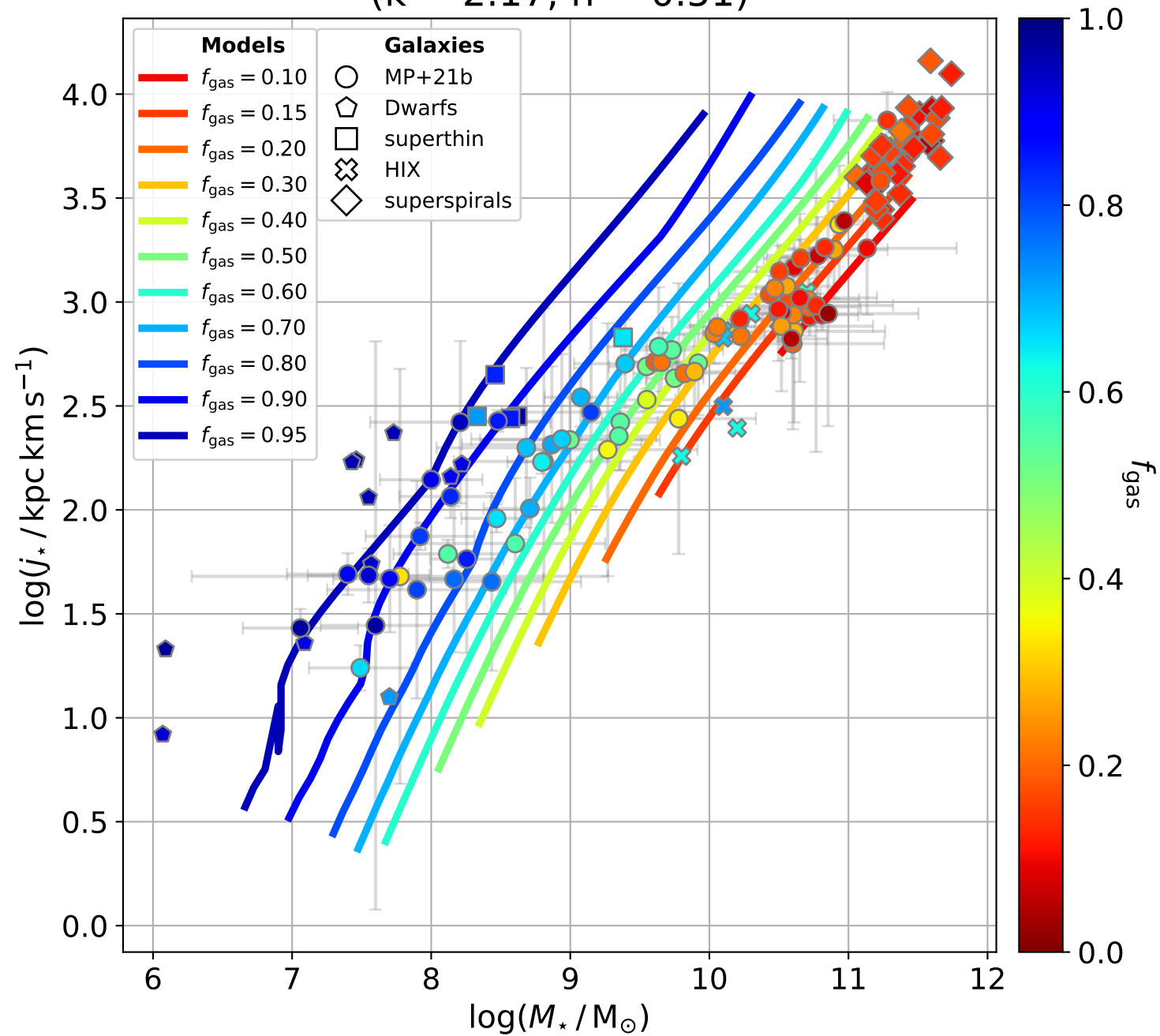
\log(j_\star) vs \log(M_\star) vs f_{\text{gas}} ( k = 2.17 , n = 0.51 )
