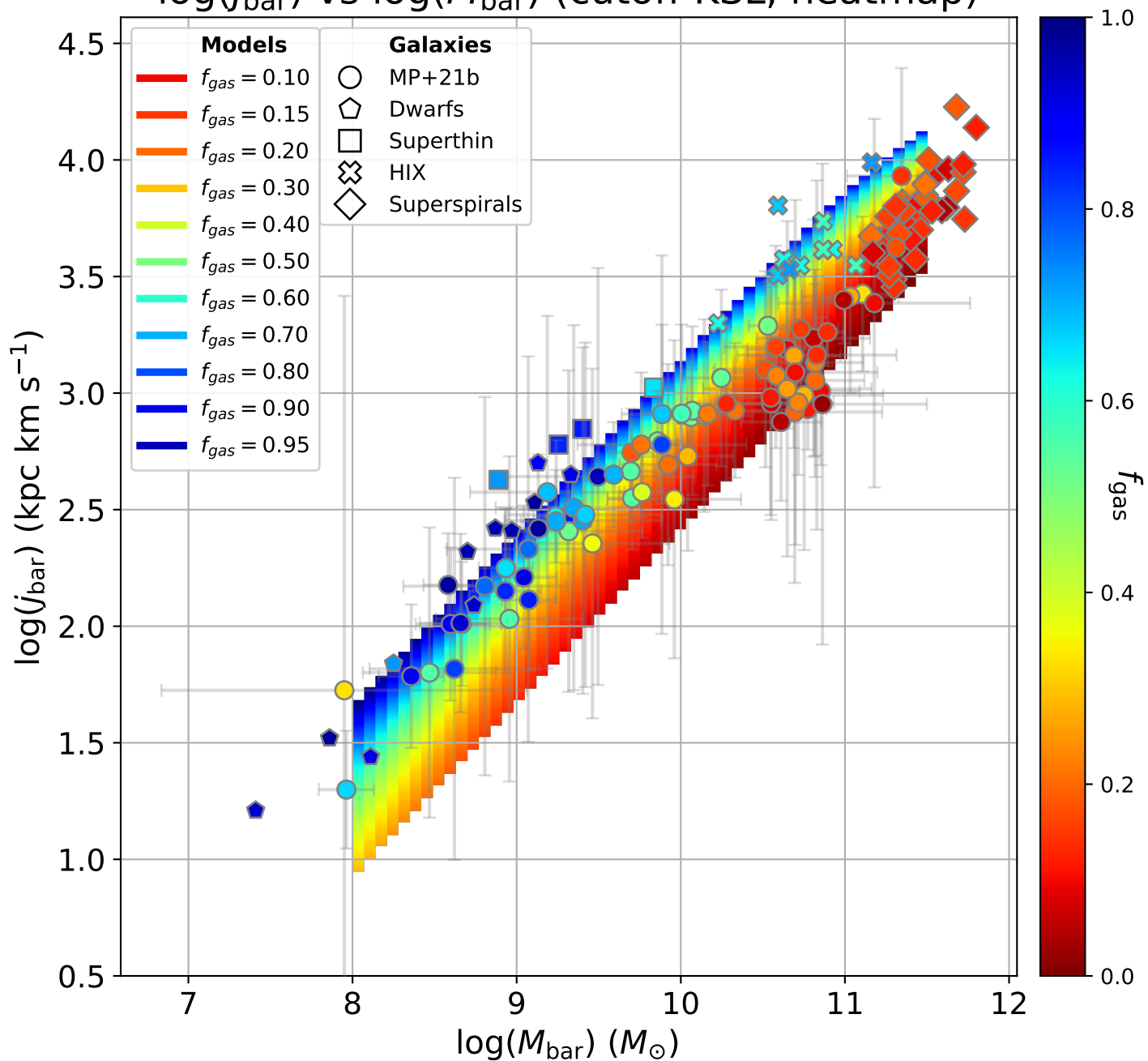
\log(j_{\text{bar}}) vs \log(M_{\text{bar}}) (cutoff KSL, heatmap)
