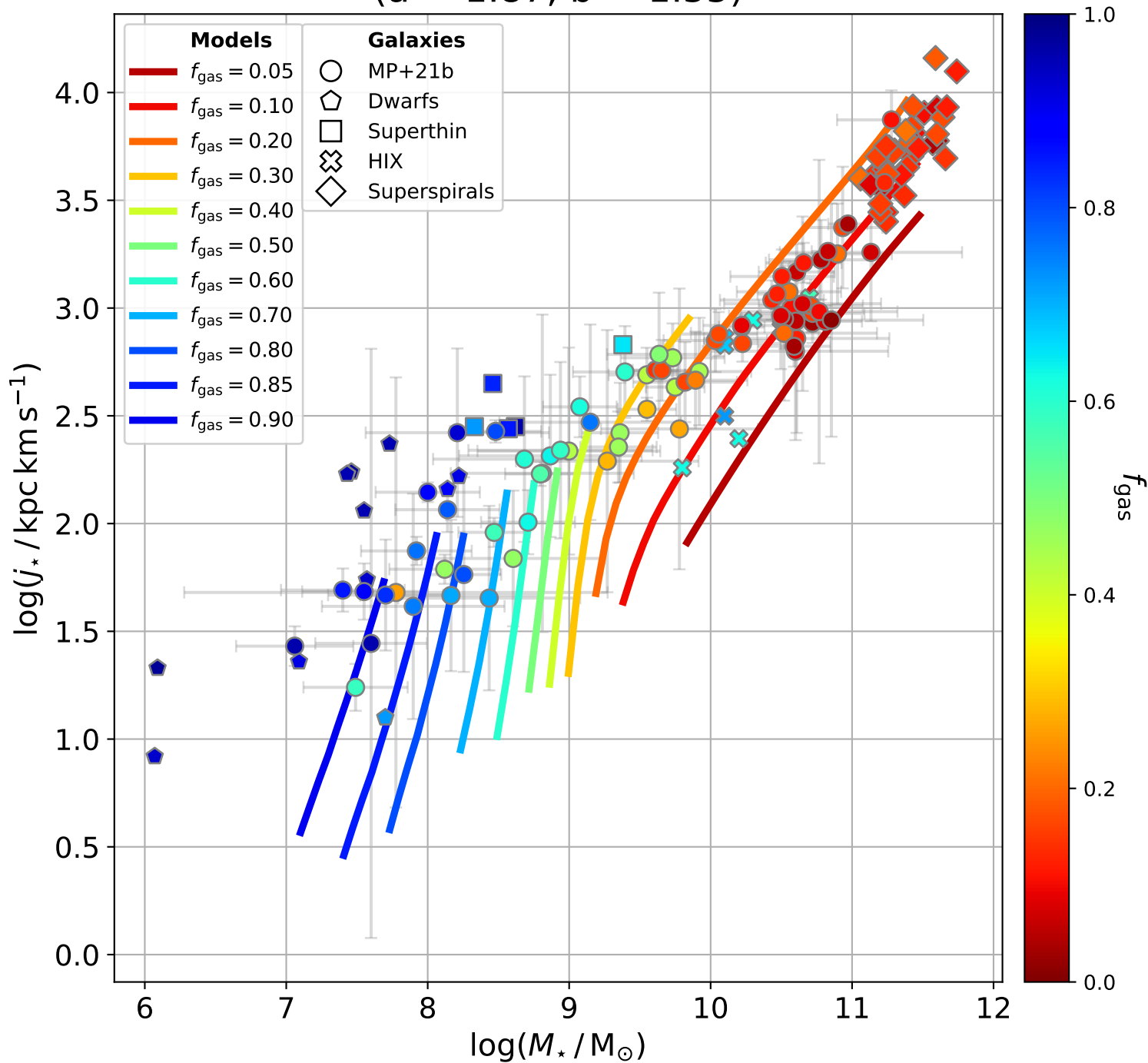
\log(j_*) vs \log(M_*) vs f_{\text{gas}} ( a = 1.87 , b = 1.55 )
