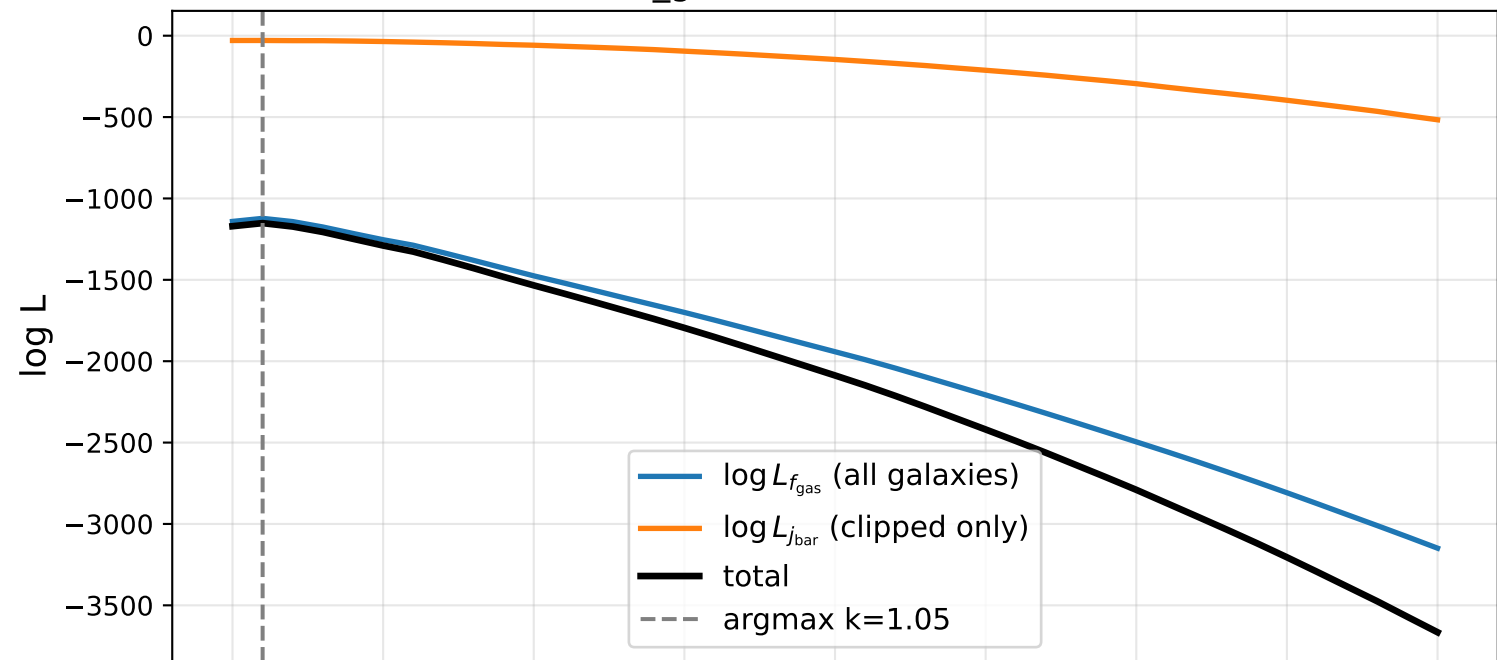
inside-out f_{\text{gas}} likelihood vs k at n = 0.354
