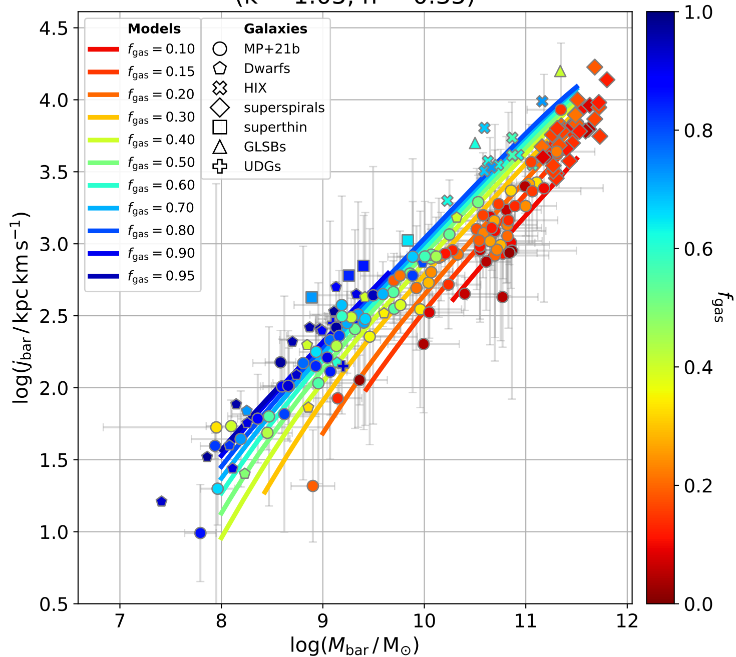
\log(j_{\text{bar}}) vs \log(M_{\text{bar}}) vs f_{\text{gas}} ( k = 1.05 , n = 0.35 )
