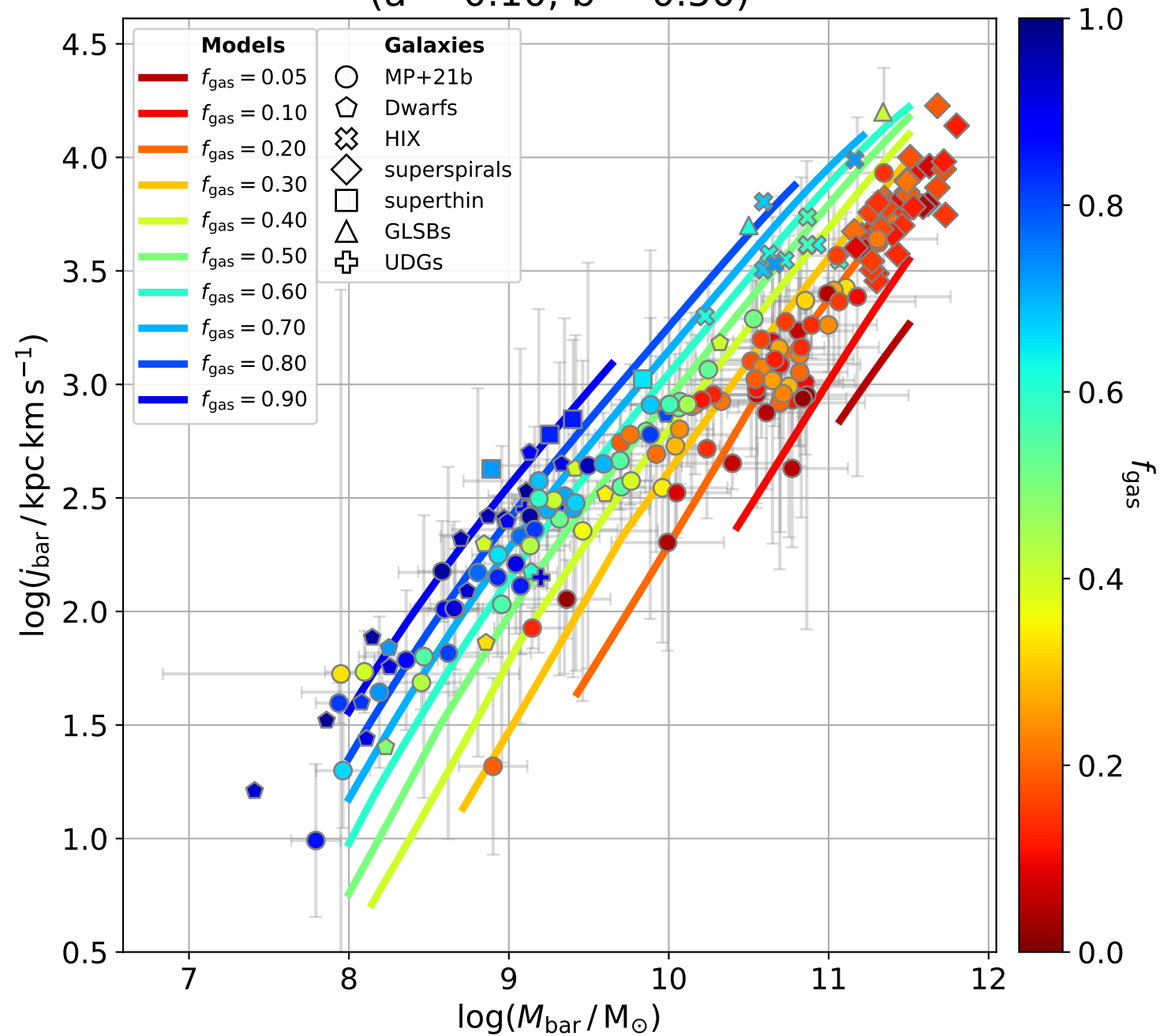
\log(j_{\text{bar}}) vs \log(M_{\text{bar}}) vs f_{\text{gas}} ( a = 0.10 , b = 0.50 )
