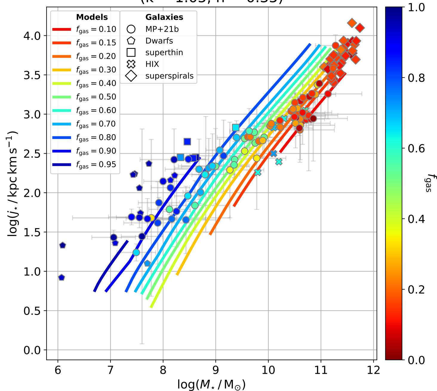
\log(j_\star) vs \log(M_\star) vs f_{\text{gas}} ( k = 1.05 , n = 0.35 )
