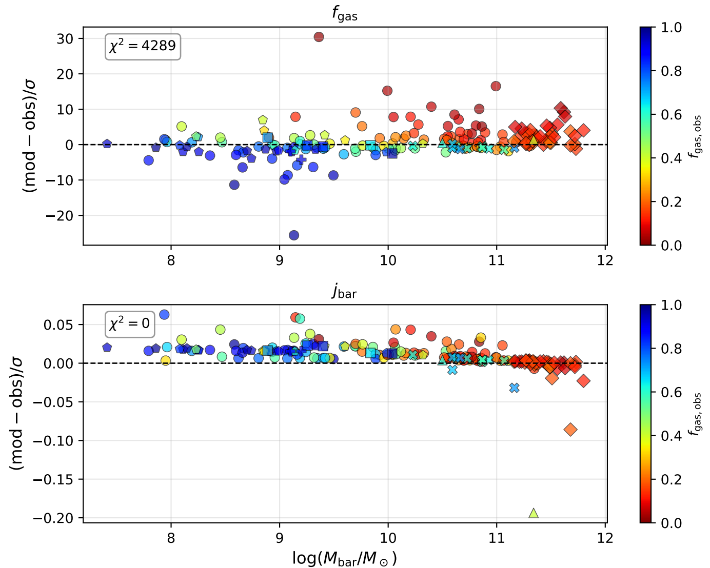
spin bias a=0.1 , b=0.5 , n=1
