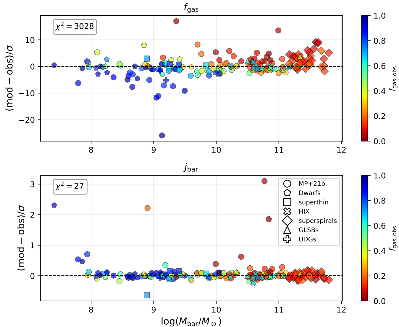
accretion bias n=1.00 , k=2.00 (clipped: 9/187)
