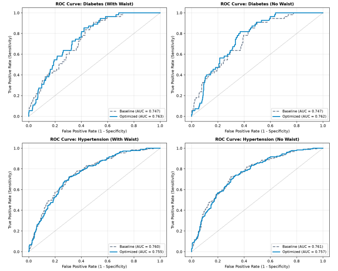
Fig. 2. Comparative ROC curves across four clinical tasks on test splits.
