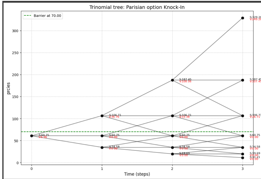
Figure 7: Parisian call up-and-in option trinomial tree
