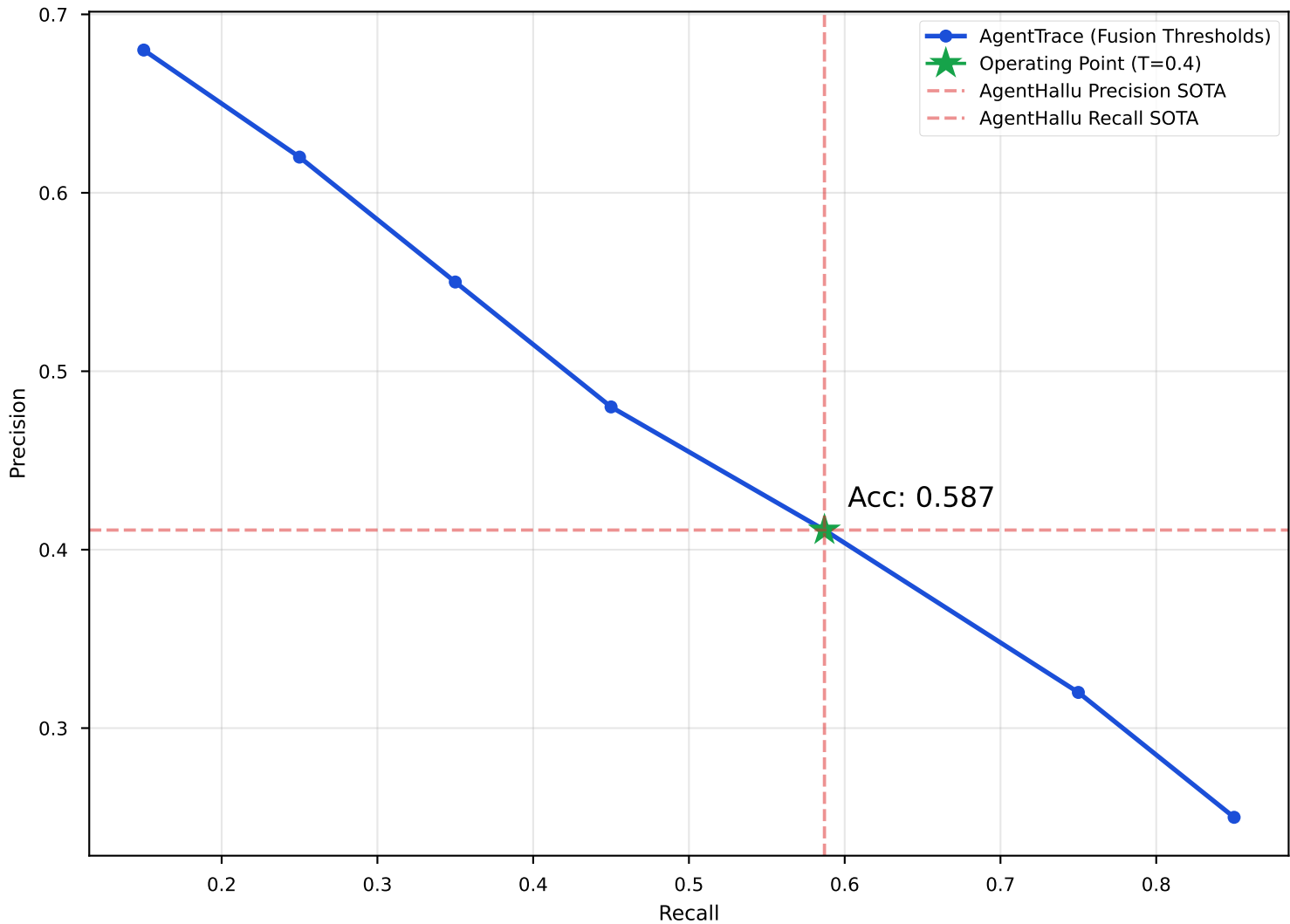
Precision vs Recall Tradeoff
